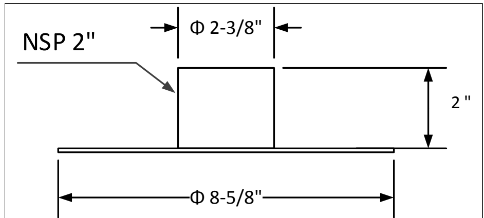
Dimensional Drawings: Side View, Units: Inches
