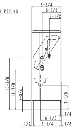
REQUIRED INSTALLATION SPACE
