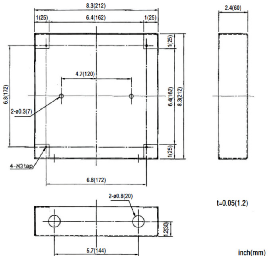
Dimensional Drawings: Units: Inches [mm]
